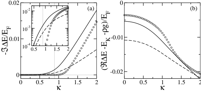
Fig. 4: For a ^{40}\text{K} impurity interacting with a Fermi sea of ^6\text{Li} ( r = 6.6439 ) on a narrow Feshbach resonance with k_{\text{F}}R_* = 1 as in [15], and k_{\text{F}}a = -0.46 . Imaginary part (a), and real part (b) of the complex energy of the impurity counted with respect to the energy of the Fermi sea, as a function of its reduced wave number \kappa = K/k_{\text{F}} . In (b) the mean-field prediction E_{\mathbf{K}} + \rho g was subtracted for clarity. Dashed (solid) lines: Perturbative calculation up to order two (three) in g . Circles: The single particle-hole ansatz. On the left of the vertical dotted line of (a) the ansatz incorrectly predicts a zero imaginary part. The inset in (a) is a magnification with the vertical axis in log-scale.
