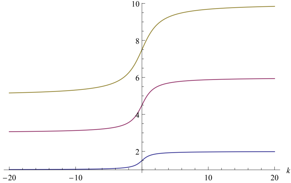
FIGURE 1. Approximative shape of the band functions k \mapsto \omega_j(k) , for j = 1, 2, 3 , of the sharp Iwatsuka Hamiltonian with b_+ = 2b_- = 2 .
