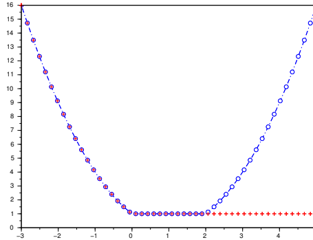
Figure 1: The graphs of the Hamiltonian p \mapsto H_i(O, p) (with the circles) and of p \mapsto H_i^+(O, p) \equiv \max_{a \in A_i: f_i(O,a) \geq 0} (-pf_i(O, a) - \ell_i(O, a)) (with the signs +). In the example, \mathcal{P}_0^i = [0, 2] .
