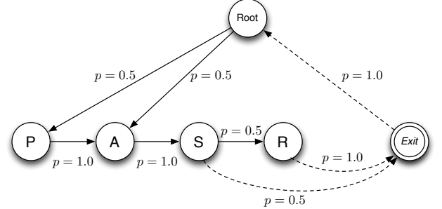
Figure 4. Topology of the PASR gesture models for 1 gesture. The prior probabilities ensure that the gesture can only be entered by the Preparation or Attack phases. Gesture models are left-to-right and reaching the exit state is only possible from the Sustain and Release phases.
