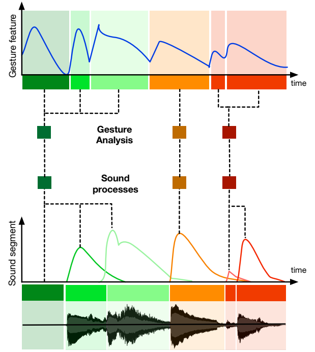
Figure 1. Overview of the proposed approach. Hierarchical structures in both gesture and sound parameters are used to build multilevel mappings from gesture to sound.
