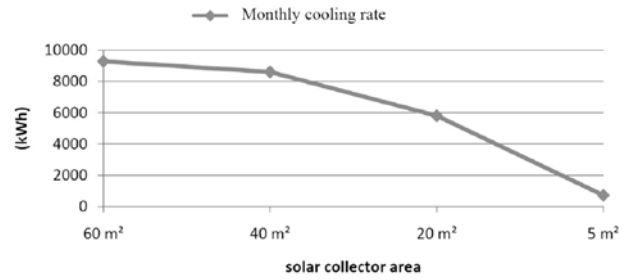
Fig. 14. Energy production from absorption chiller for different solar collector areas
