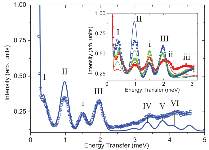
FIG. 5. (Color online) Neutron-energy loss intensity as a function of energy transfer measured on IN5 with 3.6-Å incident neutron wavelength at 2.5 K (blue circles). The blue solid line shows theoretical simulated results. The insert shows 4.0 Å incident neutron wavelength IN5 spectra at 2 (blue circles), 6 (green triangles), and 14.5 K (red squares) with simulated curves represented by solid lines. Simulations are based on (1) with exchange coupling constants of J_{CrCr} = 1.32 meV and J_{CrNi} = 3.22 meV and axial single-ion anisotropy D_{Cr} = -0.036 meV and D_{Ni} = +1.25 meV.
