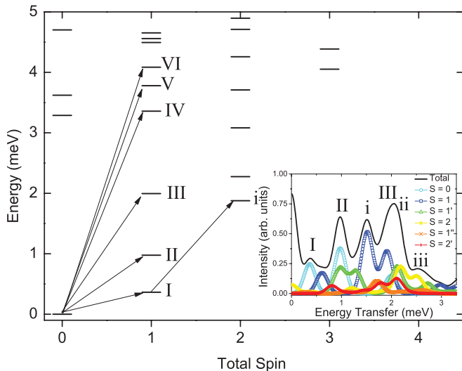
FIG. 8. (Color online) Low-lying energy spectrum for \text{Cr}_8\text{Ni} as function of total spin S , calculated with the Heisenberg-Dirac-van Vleck part of Eq. (1) using J_{\text{CrCr}} = 1.32 meV and J_{\text{CrNi}} = 3.22 meV. Labeled arrows indicate observed INS transitions. The observed hot peaks ii and iii have significant contributions from several transitions and are not indicated in the figure. The inset shows the individual contributions of the transition intensities coming from each of the low-lying spin states at 14.5 K.
