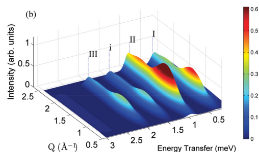
FIG. 4. (Color) (a) INS as a function of wave vector and energy transfer measured on IN5 with a 4.0-Å incident wavelength setting at 2 K. (b) Simulation based on equation (1) using exchange coupling constants J_{CrCr} = 1.31 meV and J_{CrNi} = 3.22 meV and axial single-ion anisotropy D_{Cr} = -0.036 meV and D_{Ni} = +1.25 meV.
