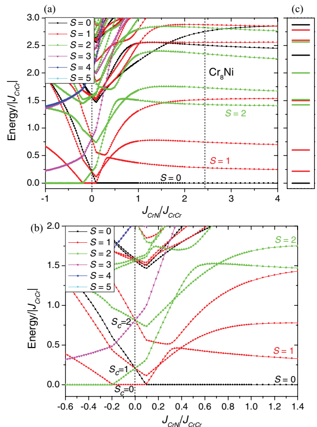
FIG. 9. (Color online) (a) and (b) show with different detail low-lying energy spectrum for \text{Cr}_8\text{Ni} as a function of the ratio J' = J_{\text{CrNi}}/J_{\text{CrCr}} , calculated with the Heisenberg-Dirac-van Vleck part of Eq. (1). (c) The low-lying energies as calculated with the effective seven-membered AFM wheel model discussed in the text. Energies are given in units of J_{\text{CrCr}} and with respect to the ground state.
