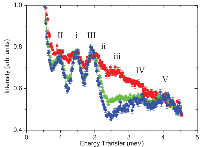
FIG. 2. (Color online) INS intensity as a function of energy transfer measured on FOCUS with a 3.5-Å incident neutron wavelength at 2 K (blue circles), 6 K (green triangles), and 18 K (red squares). Transition labels are discussed in the text.
