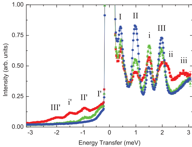
FIG. 3. (Color online) INS intensity as a function of energy transfer measured on IN5 with a 4.0-Å incident neutron wavelength at 2 K (blue circles), 6 K (green triangles), and 14.5 K (red squares). Transition labels are discussed in the text.
