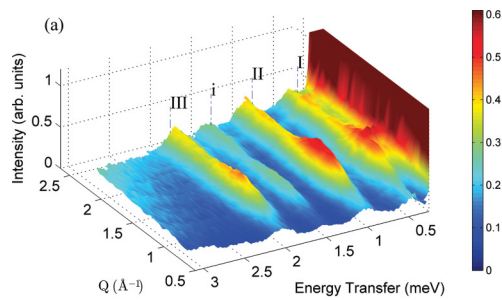
FIG. 4. (Color) (a) INS as a function of wave vector and energy transfer measured on IN5 with a 4.0-Å incident wavelength setting at 2 K. (b) Simulation based on equation (1) using exchange coupling constants J_{CrCr} = 1.31 meV and J_{CrNi} = 3.22 meV and axial single-ion anisotropy D_{Cr} = -0.036 meV and D_{Ni} = +1.25 meV.
