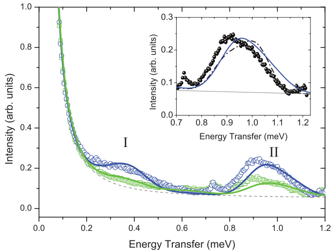
FIG. 6. (Color online) INS intensity as a function of energy transfer measured on IRIS. The blue open circles and green open squares show 1.5 and 6 K spectra, respectively. Solid lines show simulated spectra based on (1) with exchange coupling constants of J_{\text{CrCr}} = 1.32 meV and J_{\text{CrNi}} = 3.22 meV, and axial single-ion anisotropy D_{\text{Cr}} = -0.036 meV and D_{\text{Ni}} = +1.25 meV. The broken line represents the elastic line and background contributions of the simulated spectra. The insert shows the 1.5 K spectrum near feature II in more detail (black circles) and the solid blue line represents the simulation using D_{\text{Ni}} = +1.25 meV and the dash-dotted black line that for D_{\text{Ni}} = -0.43 meV.
