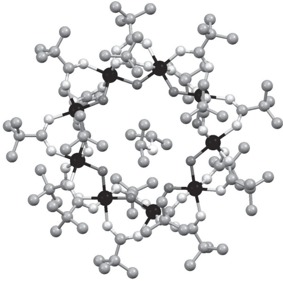
FIG. 1. The Structure of the \text{Cr}_8\text{Ni} . Cr and Ni ions are represented by large black spheres, where the Ni position is disordered over the nine possible metal sites, O are light gray spheres, C gray spheres, F dark gray spheres, and N in the center of the wheel is represented by a white sphere. H atoms are omitted for clarity.
