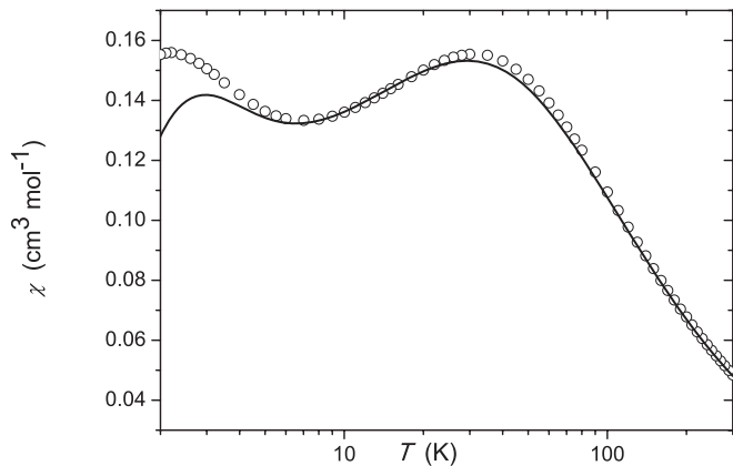
FIG. 7. The molecular susceptibility of \text{Cr}_8\text{Ni} (black circles) at 1 KOe, measured in a temperature range of 2 to 300 K. The black solid line shows theoretical calculated results based on Eq. (1) using the exchange constants determined from the INS experiments, J_{\text{CrCr}} = 1.32 meV, J_{\text{CrNi}} = 3.22 meV, and Zeeman terms with g_{\text{Cr}} = 1.98 and g_{\text{Ni}} = 2.2 .
