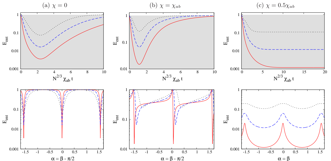
FIG. 6: (Color online) Top row: evolution of the entanglement witness E_{\text{ent}} (41) for three different ratios \chi/\chi_{ab} . The number of atoms in each ensemble is N = 50 (black dotted line), N = 500 (blue dashed line), and N = 5000 (red solid line). The quadrature angle \alpha has been optimized numerically, while \beta is fixed by the conditions (34),(37),(38). Bottom row: dependence of E_{\text{ent}} on the angle \alpha while \beta is still given by the conditions (34),(37),(38). In these curves the time is fixed to the best time (minimum of E_{\text{ent}} ) extracted from the top row curves.
