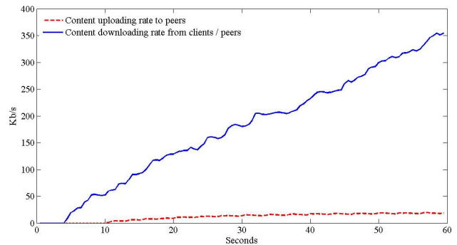
Fig. 7. Active tracker (random chunk): Uploading/Downloading rates
