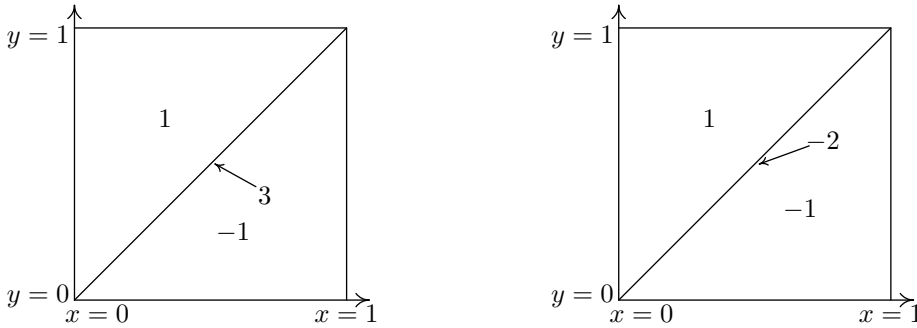
Figure 1: Representation of u_1(x, y) of type A and B.
