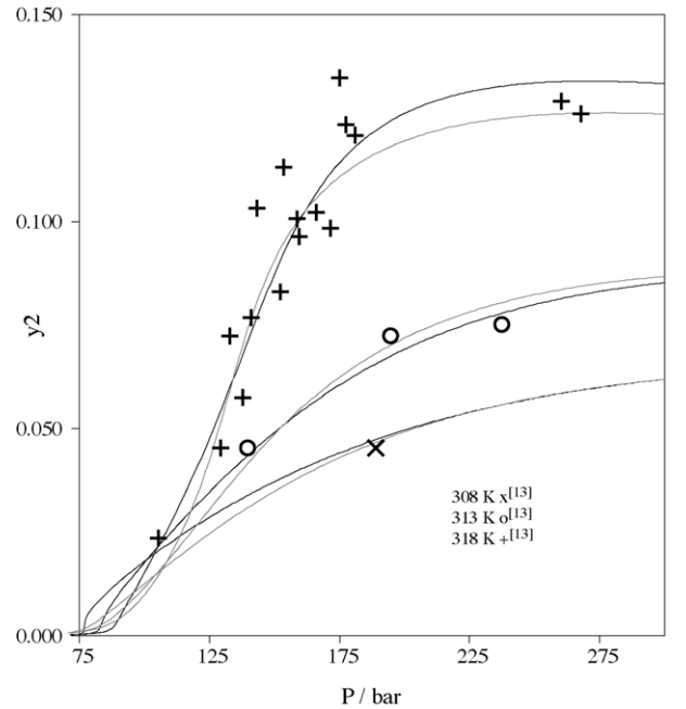
Fig. 6. Solubility of naphthalene(2) in xenon. Correlation using “ k_{ij}(T), l_{ij} ” mixing rule with: – Sanchez–Lacombe EoS (Table 7), ... Peng–Robinson EoS ( k_{12}' = 0.0087 , k_{12}'' = 0.1192 , l_{12} = -0.0292 ).
