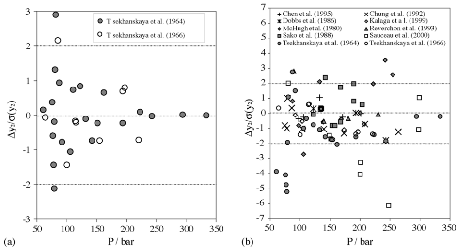
Fig. 2. Carbon dioxide–naphthalene system: deviations \Delta y_2/\sigma(y_2) between experimental and estimated values of solubility (Eq. (A.1)). (a) Correlation of single data sets at 308.15 K in step (1). (b) Correlation of the whole data set at 308.15 K in step (2).
