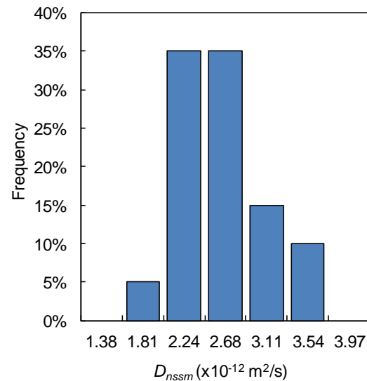
Figure 7 – Histogram of the migration coefficient for the A2-2 series.
