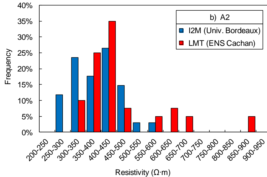
Figure 12 – Resistivity distribution for concrete A2 (the specimens used at I2M were 90 days old whereas the age was 1 year at LMT).
