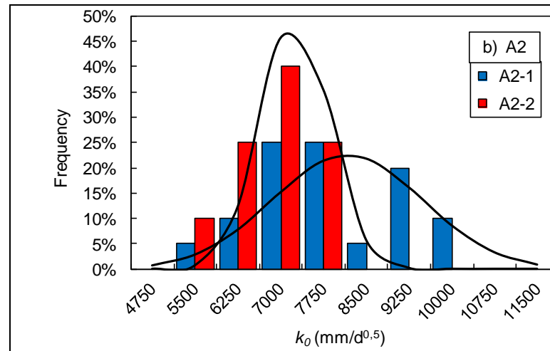
Figure 20 – Accelerated degradation kinetics distribution (using ammonium nitrate). The solid lines are guides for the eyes only (normal probability density function).
