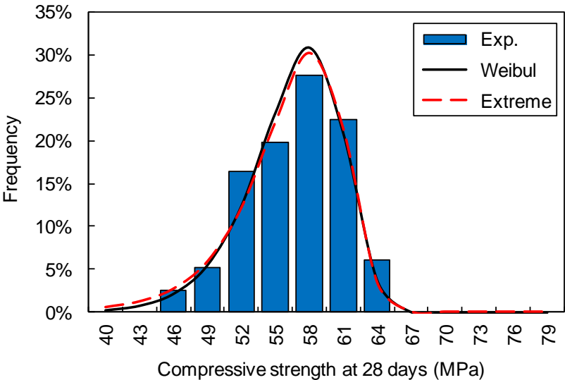
623 Figure 23 – Experimental (cf. Figure 4) and theoretical probability densities and distribution functions for the compressive strength of A1 624 concrete at 28 days (sample size: 116).
