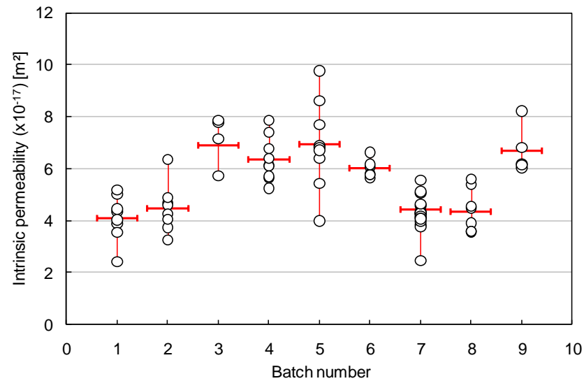
Figure 21 – Intrinsic permeability (using nitrogen) of the first nine batches (construction site A1). Each circle corresponds to an experimental value obtained using a cored specimen. The horizontal bar stands for the mean value for each batch.
