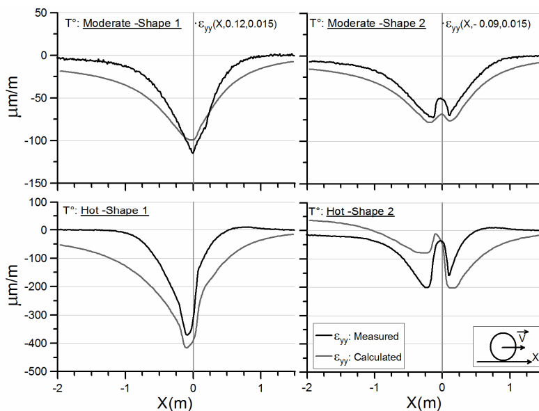
Figure 5: Transverse strain for two temperatures (structure A) at Z= 15 mm
