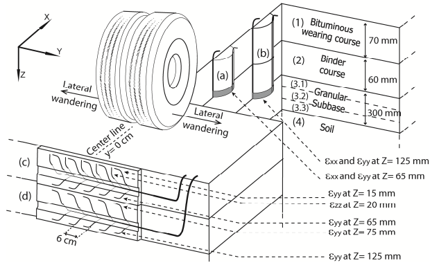
Figure 1: Configuration and instrumentation of the structure A (two instrumented concrete cores (a and b) and two instrumented polymeric plates (c and d))
