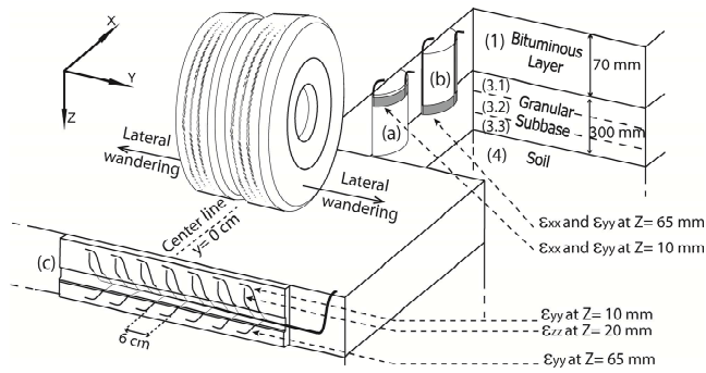
Figure 2: Configuration and instrumentation of the structure B (two instrumented concrete cores (a and b) and one instrumented polymeric plate (c))
