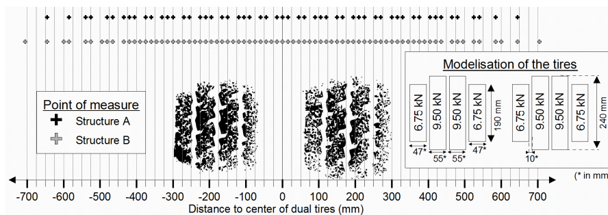
Figure 3: Distribution of measurement points under the footprint of the tire.
