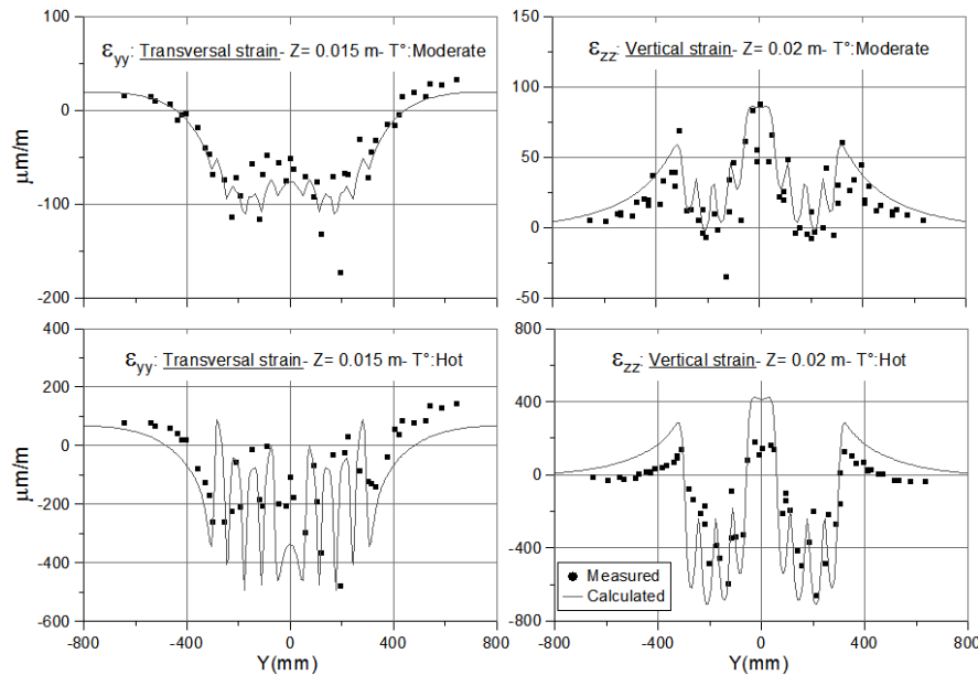
Figure 7: Measured and computed strain basins for two temperatures (structure A)
