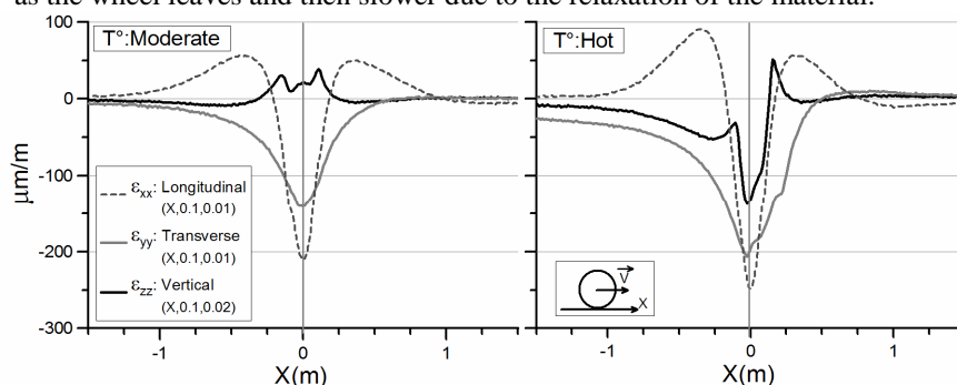
Figure 4: Strains near the surface for two temperatures (plan y=100 mm)
