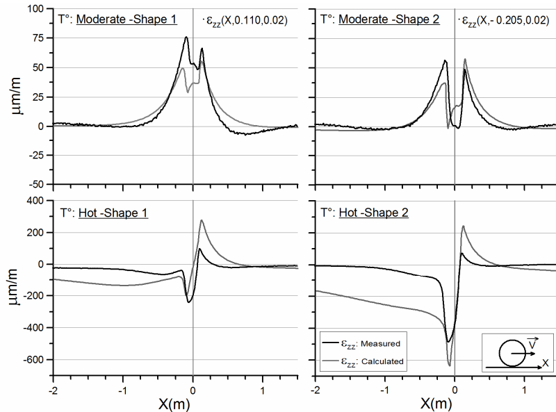
Figure 6: Vertical strain for two temperatures (structure A) at Z=20 mm
