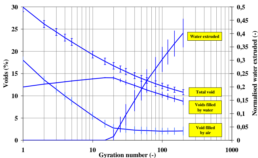
Figure 3 – Gyratory shear compactor densification (embarked GSC2)
