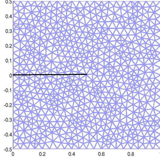
Figure 6: Unstructured mesh.
