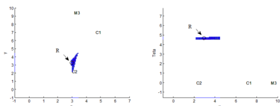
Figure 7: 3-DOF robot localization (x,y) in meters and \theta in radians. a) Projection in the x - y plane, b) Projection in the y - \theta plane.
