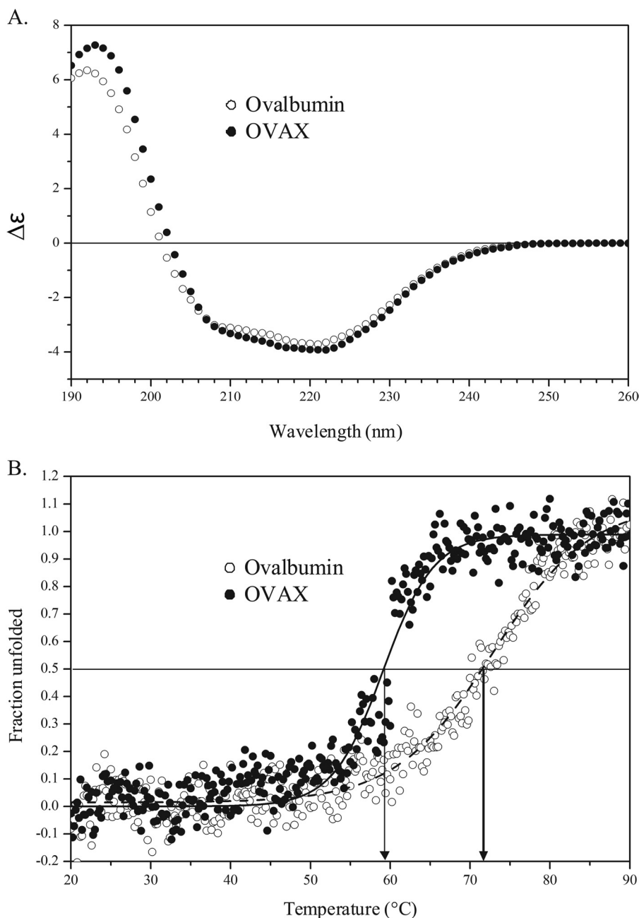
FIGURE 7. Circular dichroism analyses of OVAX and ovalbumin proteins. A , far-UV CD spectra of OVAX (filled circles) and ovalbumin (empty circles). The unit on the ordinate is mean differential absorption coefficient ( \Delta\epsilon ). B , thermal denaturation of OVAX (filled circles) and ovalbumin (empty circles) monitored by following the changes in ellipticity at 222 nm.
