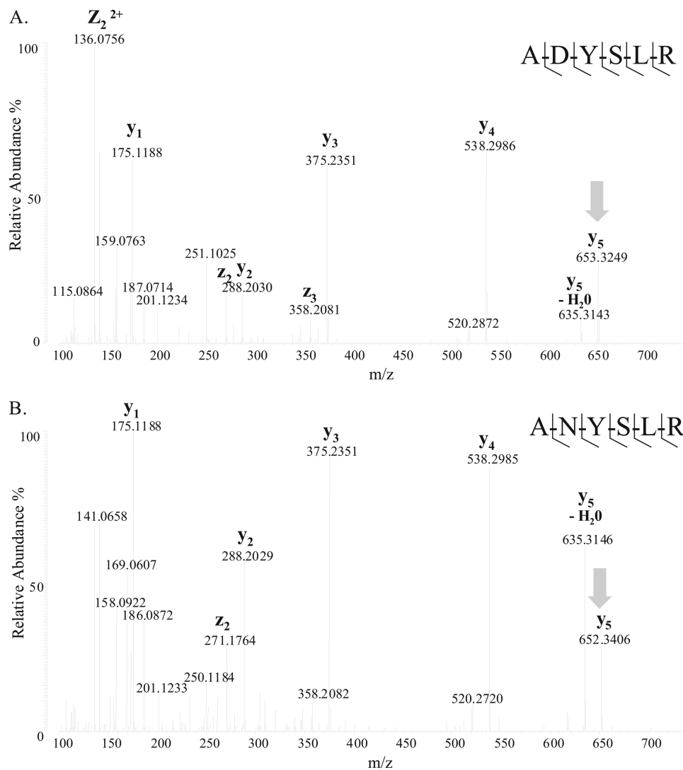
FIGURE 5. Heterogeneity of Asn 102 glycosylation site. A, MS/MS spectrum assigned to the deglycosylated OVAX peptide. The bicharged precursor ion ( m/z 362.6849 [ M + H ] + = 724,3551) was isolated and fragmented by higher-energy collisional dissociation. Fragment ions containing the C terminus ( y - and z -type ions) are labeled. The characterization of the N -deamidation (+0.98402) by the observed y_5 fragment ion ( m/z 653,3249; gray arrow) confirmed the conversion of asparagine to aspartate by the PNGase F and therefore the site of glycosylation on Asn 102 . B, MS/MS spectrum assigned to non-glycosylated ANYSLR peptide (bicharged precursor ion ( m/z 362,1930, [ M + H ] + = 723,386) showing post-translational modifications heterogeneity within OVAX.
