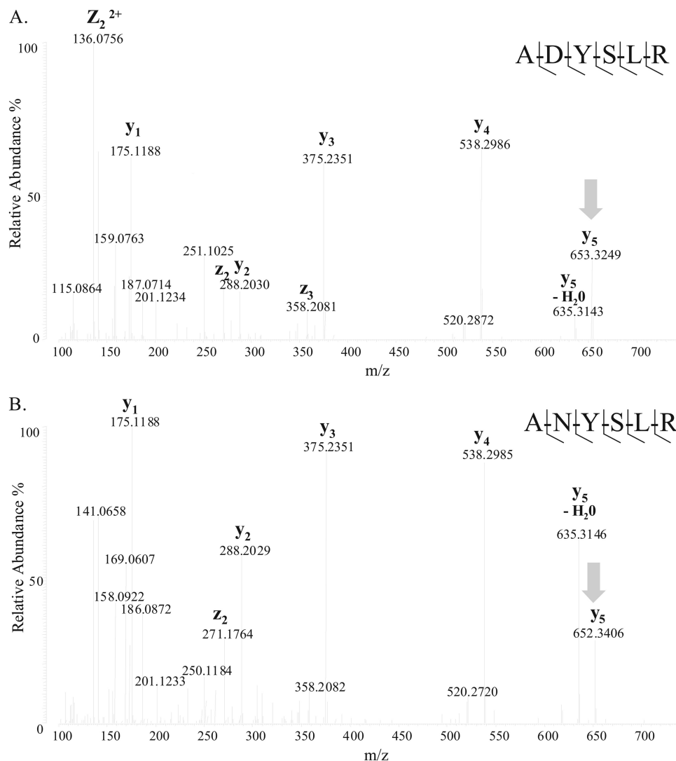
FIGURE 5. Heterogeneity of Asn 102 glycosylation site. A, MS/MS spectrum assigned to the deglycosylated OVAX peptide. The bicharged precursor ion ( m/z 362.6849 ( [M + H]^+ = 724,3551 )) was isolated and fragmented by higher-energy collisional dissociation. Fragment ions containing the C terminus (y- and z-type ions) are labeled. The characterization of the N-deamidation (+0.98402) by the observed y_5 fragment ion ( m/z 653,3249; gray arrow) confirmed the conversion of asparagine to aspartate by the PNGase F and therefore the site of glycosylation on Asn 102 . B, MS/MS spectrum assigned to non-glycosylated ANYSLR peptide (bicharged precursor ion ( m/z 362,1930, [M + H]^+ = 723,386 )) showing post-translational modifications heterogeneity within OVAX.
