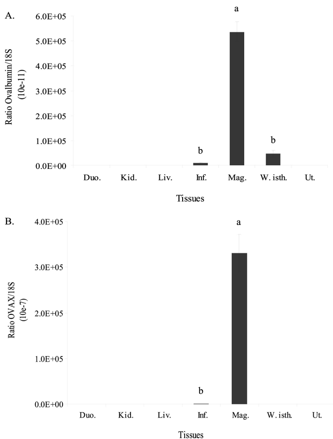
FIGURE 1. Tissue expression of ovalbumin (A) and OVAX (B) in chicken hens. Means that do not share a common letter are significantly different ( p < 0.05 ; n = 8 ). Duo., duodenum; Kid., kidney; Liv., liver; Inf., infundibulum; Mag., magnum; W. Isth., white isthmus; Ut., uterus. Ratio are expressed as arbitrary units.
