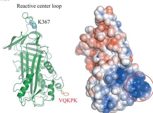
FIGURE 8. Modeling of OVAX from the three-dimensional structure of ovalbumin. A, ovalbumin. Left panel, schematic representation of the three-dimensional structure of ovalbumin (purple). The disulfide bond between Cys 73 and Cys 120 is indicated in yellow. Right panel, electrostatic potentials mapped over the molecular surface of ovalbumin. B, OVAX. Left panel, schematic representation of the three-dimensional structure model of OVAX (green). The OVAX pentapeptide VQKPK is highlighted in red. Right panel, electrostatic potentials mapped over the molecular surface of OVAX. The red circle highlights the putative heparin binding area. P1 reactive sites are Ala 358 for ovalbumin and Lys 367 for OVAX.
