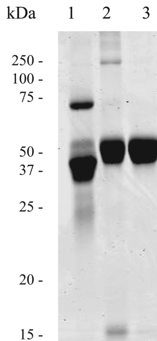
FIGURE 2. Purification of a heparin-binding protein from egg white. Lane 1, egg white; lane 2, heparin-binding proteins from egg white; lane 3, purified OVAX. Samples were analyzed by SDS-PAGE followed by Coomassie Blue staining.
