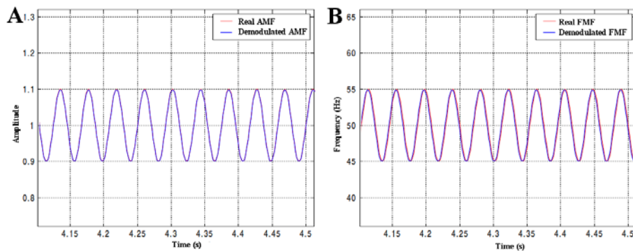
Figure 9. The non-harmonic overlapping condition is not verified. The amplitude ratio between the sidebands of the fundamental and those of its first harmonic is large.
