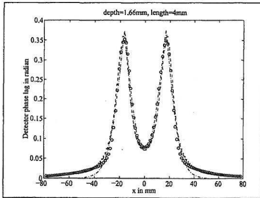
Figure 3. Observations (o) and mean-square fitted curves for the models 1 (.), 2 (- -) and 3 (-.-).
