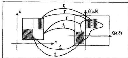
Figure 1. Inclusion function f_{\square} of a function f .
