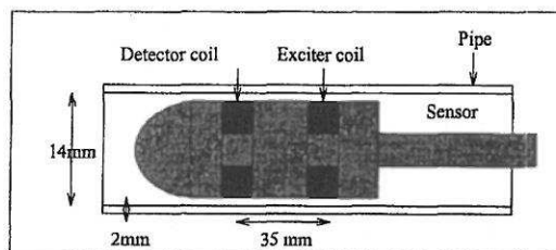
Figure 2. Schematic illustration of the sensor pipe.
