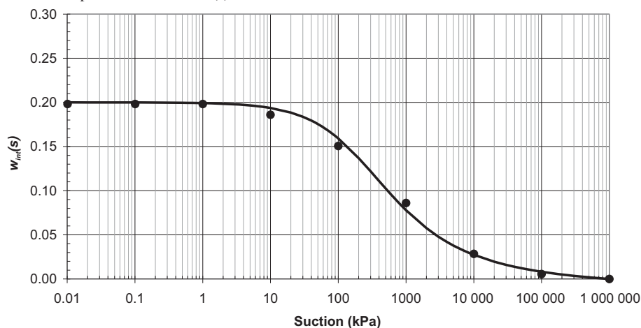
Fig. 10. Evolution of the intercept water content w_{\text{int}}(s) with suction.
