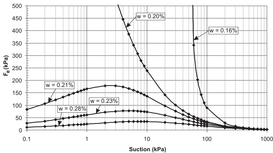
Fig. 16. Evolution of F_e with suction for different constant values of water content.
