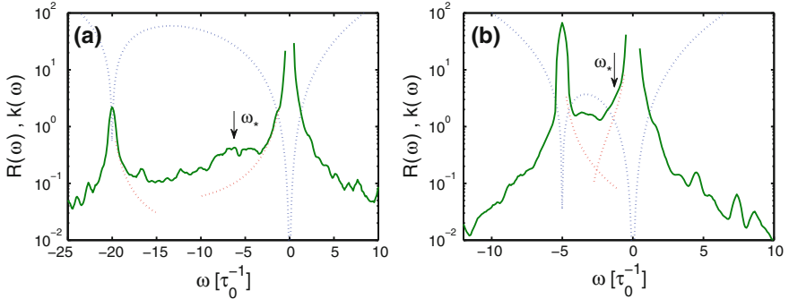
Figure 5. Applicability criterion of the wave turbulence theory, \mathcal{R}(\omega) = k_{nl}(\omega)/k(\omega) \ll 1 , for two cases considered in Figure 2: a \alpha = 0.05 , b \alpha = 0.2 . The function \mathcal{R}(\omega) is plotted in logarithmic scale, it has been obtained by averaging the NLS spectrum from z = 2,500 to z = 2,550 (over 50 realizations, \sigma = 1 ). The dashed blue line shows the dispersion relation |k(\omega)| , the arrows indicate the location of the zero-dispersion frequency \omega_* (color figure online).
