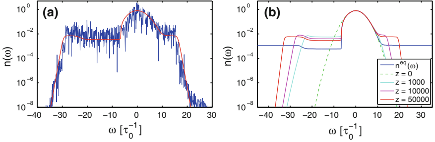
Figure 7. a Second stage of the spectral evolution obtained by integrating numerically the NLSE (34) (blue) and the kinetic (38) (red) at z=20,000 for \alpha=0.05 ( \sigma=1 ). b Numerical simulations of the kinetic (38) showing the spectral profile n(z, \omega) at different propagation lengths z : a constant spectral pedestal emerges in the tails of the spectrum ( \alpha=0.05 ). The spectrum slowly relaxes toward the equilibrium state n^{\text{loc}}(\omega) given by (39) (blue) (color figure online).
