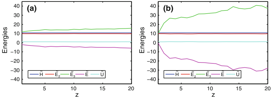
Figure 4. Evolutions of the densities of the Hamiltonian \tilde{H} = H/T_0 , of the kinetic energy \tilde{E} = E/T_0 , of the nonlinear energy \tilde{U} = U/T_0 , and of the quadratic \tilde{E}_2 = E_2/T_0 and cubic \tilde{E}_3 = E_3/T_0 energy contributions to the kinetic energy, for \alpha=0.05 (a), and \alpha=0.2 (b) ( T_0 is the size of the numerical temporal window). a and b correspond to the first and third columns reported in Figure 2.
