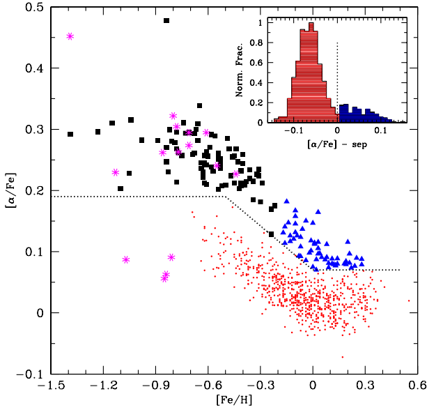
Fig. 1. [\alpha/\text{Fe}] vs. [\text{Fe}/\text{H}] for the whole sample. Magenta asterisks represent the stars belonging to the halo by their kinematics. The black dotted line is the fiducial for division into thin- and thick disk populations. The black filled squares refer to the thick disk stars, blue triangles to the h\alpha mr, and the red dots to the thin disk stars. On the top-right corner we plot the histogram of the distribution of [\alpha/\text{Fe}] , after the fiducial model (separation curve) is subtracted.
