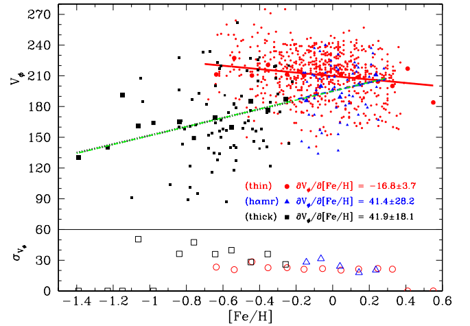
Fig. 4. Galactic rotational velocity gradients (filled symbols) and velocity dispersion gradients (open symbols) with metallicity for stars assigned to different stellar populations. The symbols are the same as in previous plots. The smaller symbols correspond to the real stars and the larger symbols represent the V_\phi and \sigma_v values for metallicity bins. Note that the slopes are obtained for the full unbinned data.
