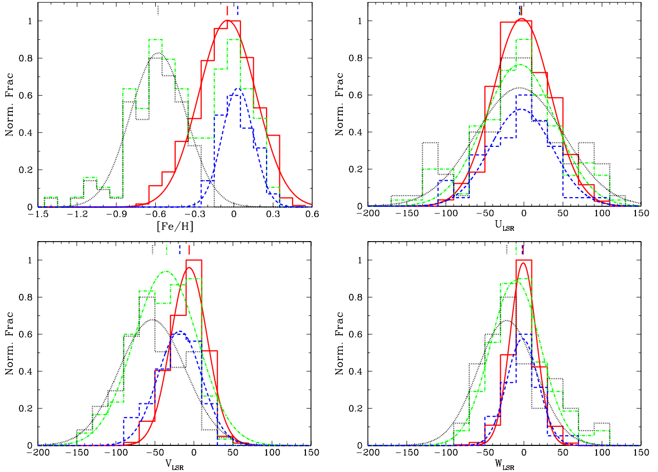
Fig. 2. Distributions of the Galactic space velocities and metallicity of the stars from the thick disk (black dotted), h\alpha mr (blue dashed), the thin disk (red solid), and the thick disk + h\alpha mr (green dot-dashed). Gaussian fits of the data are also presented. The mean of Gaussian fits is shown by vertical lines at the top of each distribution. Note that the distributions of different groups were set lower or higher for the sake of clarity.
