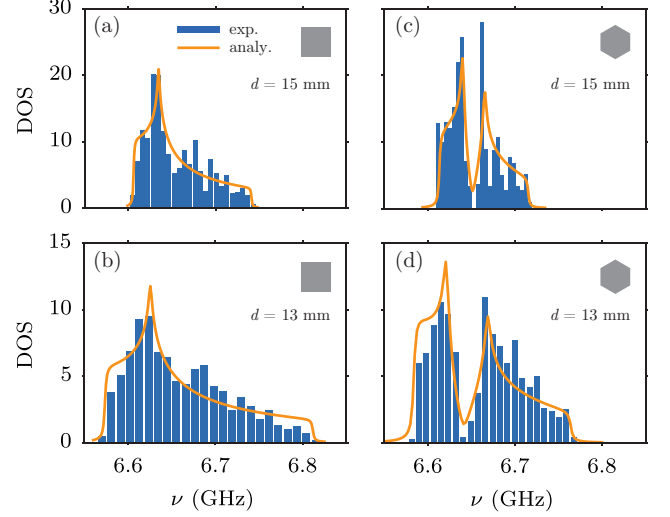
FIG. 8. DOS for regular square (a,b) and hc (c,d) lattices for various lattice constant d . (a,c) d = 15 mm. (b,d) d = 13 mm. Blue area: Normalized histogram with 24 bins per bandwidth (see text for details) of the g function averaged over all the position \mathbf{r} . Orange line: Analytical solution for a infinite system taking into account the N1, N2 and N3 coupling terms. These parameters are obtained by locating the points of interest as seen in Fig. 7.
