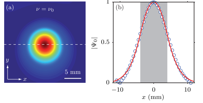
FIG. 2. (Color online) Isolated resonator response. (a) Normalized experimental wave function intensity |\Psi_0|^2 at the frequency \nu_0 = 6.65 GHz. (b) Profile of |\Psi_0| corresponding to the dashed line in (a). The gray zone is the disc position. Red curve: Fit from equation (2) with \gamma_j = 0.3341 \text{ mm}^{-1} , \gamma_{k,1} = 0.1215 \text{ mm}^{-1} , \gamma_{k,2} = 0.3423 \text{ mm}^{-1} , and \gamma_{k,3} = 0.5366 \text{ mm}^{-1} and \alpha_1 = -0.1370 , \alpha_2 = 5.3816 , and \alpha_3 = -6.6585 .
