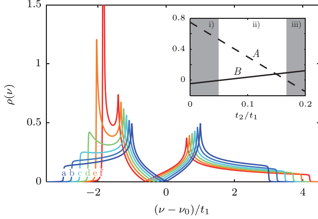
FIG. 9. Density of states for t_2/t_1 = 0.0 (a), 0.04 (b), 0.08 (c), 0.12 (d), 0.16 (e), and 0.2 (f) with t_1 = -1 and t_3 = 0 . The DOS is calculated numerically without broadening. Inset: A and B parameters versus t_2/t_1 .
