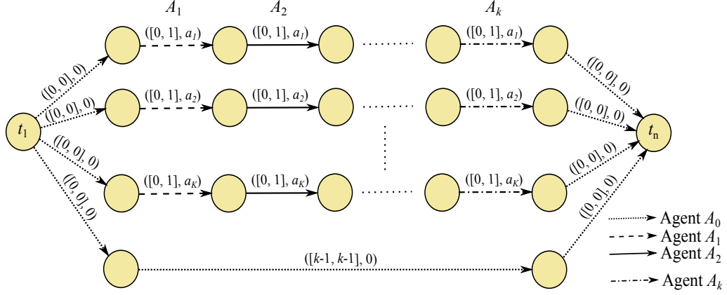
Figure 3 Reduction from 3-PARTITION problem
