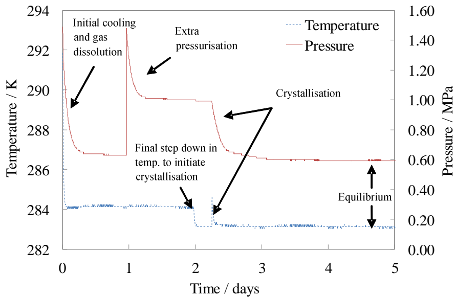
Figure 1. Typical recording of temperature and pressure as functions of time during experimental start-up and hydrate crystallisation. Recording from experimental run in equilibrium cell C1. Formed hydrate is a mixed THF/CO 2 hydrate. (Dotted line) Temperature / K, (Full line) Pressure / MPa.
