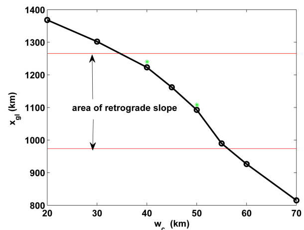
Fig. 6. Stable grounding-line positions along the medial line as a function of channel half-width. The data points shown as black circles are based on results obtained using \acute{U}a . The data points shown as green stars were obtained with Elmer/Ice.
