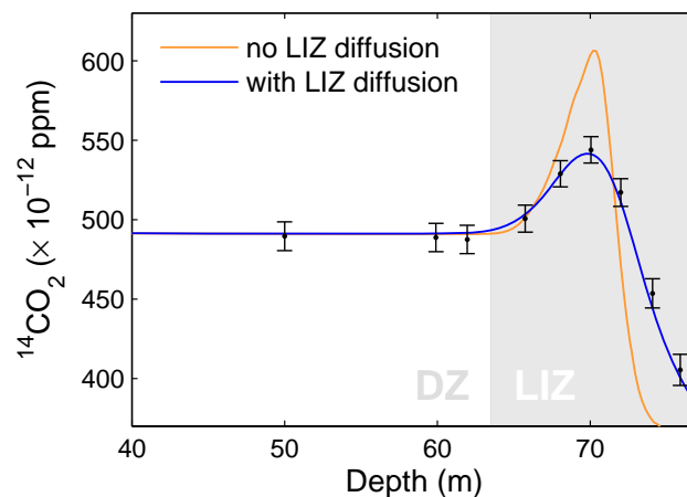
Fig. 6. Modeled 14 CO 2 profiles both with, and without diffusivity in the LIZ. Calculations done with the CIC firn air model.
