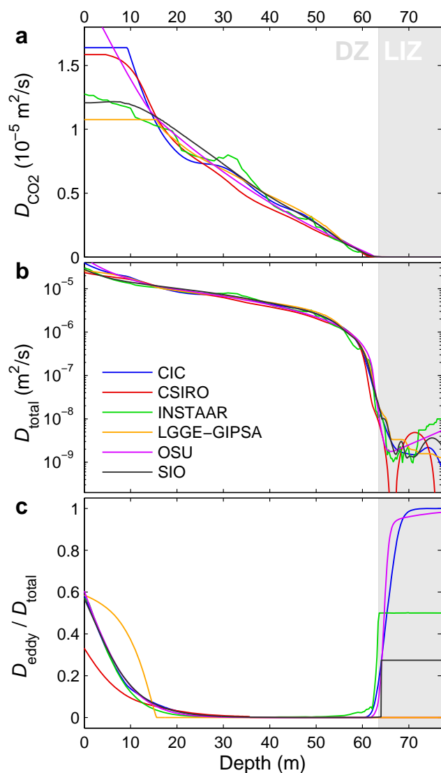
Fig. 5. (a) CO 2 molecular diffusivity profile with depth D_{\text{CO}_2}(z) for the EU borehole. (b) Semi-log plot of the total CO 2 diffusivity profile D_{\text{total}}(z) = D_{\text{CO}_2}(z) + D_{\text{eddy}} . (c) Plot of D_{\text{eddy}}(z)/D_{\text{total}}(z) . Eddy diffusion near the surface corresponds to convective mixing; in the LIZ some of the models include dispersive mixing. The CSIRO model has zero eddy diffusivity in the LIZ; the line is not visible as the LGGE-GIPSA model is plotted on top of it.
