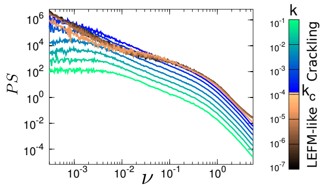
FIG. 3. (Color online) Power spectrum (PS) of \bar{v}(t) obtained for various value of k (logarithmic axes). Other parameters are kept constant: c = 10^{-5} , N = 1024 and \sigma = 1 . Right-handed colorbar indicates the k value. Note the qualitative change at the transition k_c , and the power-law observed above, in the crackling regime.
