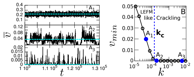
FIG. 1. A1→A3: Time evolution of the spatially averaged crack front velocity \bar{v}(t) for increasing unloading factor k : k = 4.75 \times 10^{-5} (A1), k = 2 \times 10^{-4} (A2) and k = 5.5 \times 10^{-3} (A3). Other parameters are kept constants: c = 10^{-5} , N = 1024 and \sigma = 1 . At low k , \bar{v}(t) wanders around the value c/k expected in absence of microstructural disorder, with relative fluctuations that decreases with k . For higher k , the dynamics become jerky and, above a given value k_c , separated pulses can be distinguished, which sharpens as k increases. B: Minimum value of \bar{v}(t) vs. k . The transition value k_c between CM-like and crackling dynamics is precisely defined as the smallest value k for which v_{min} = 0 .
