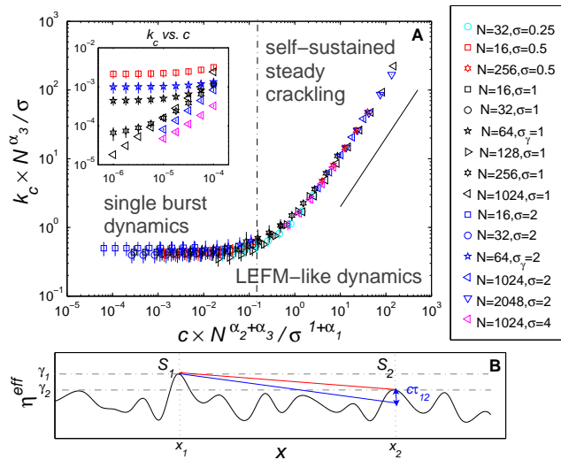
FIG. 2. (Color online) A: Phase diagram of the crack dynamics. Inset: variation of k_c as a function of c for different N and \sigma (values on right-hand side). Each point results from averaging over many simulations and errorbars correspond to a 95% confidence interval. Main panel: Collapse obtained using Eq. 4 with \alpha_1 = 0.38 , \alpha_2 = 1.15 and \alpha_3 = 1.65 . Straight line indicates proportionality. In both graphs, the axis are logarithmic. B: Sketch of the variation of the effective pinning force applying on the front as it quasistatically propagates throughout the disordered landscape (see e.g. [30] for implementation of such a propagation algorithm). Points S_1 = \{x_1, \eta_1\} and S_2 = \{x_2, \eta_2\} locate the maximum and following next-to-maximum peaks over the traveled distance (see text for details).
