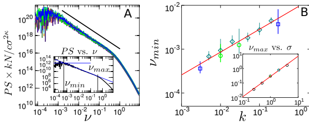
FIG. 4. (Color online) A(main panel): Collapsed PS curves of \bar{v}(t) in the self-sustained steady crackling part of the phase diagram (logarithmic axes). The collapse is obtained using Eq. 5 with \kappa = 0.7 . The different curves (with different colors) correspond to different values of c, k, N, \sigma : 10^{-6} \leq c \leq 3 \times 10^{-4} , 3 \times 10^{-3} \leq k \leq 3 \times 10^{-2} , 128 \leq N \leq 2048 , \sigma = 1 . Black straight line is a power law of exponent 1/a = 1.5 . A(inset): For a given PS(\nu) curve, \nu_{min} is defined from the intersection of the power-law and the plateau value at low frequencies, while \nu_{max} sets the upper cutoff for the power-law. B(main panel): Variation of the lower cutoff \nu_{min} with k for c = 10^{-5} ( \circ ), c = 3 \times 10^{-5} ( \square ), c = 3 \times 10^{-5} ( \diamond ), and constant values N = 1024 and \sigma = 1 [It was checked that \nu_{min} is independent of both N and \sigma ]. In both plots, straight lines are power-law (Eq. 6) with 2\kappa = 1.4 , and \Delta = 0.52 . B(inset): Variation of the upper cutoff \nu_{max} with \sigma for N = 128 ( \square ), N = 256 ( \triangle ), N = 1024 ( \circ ), N = 2048 ( \diamond ) and constant values c = 10^{-5} and k = 10^{-3} [It was checked that \nu_{max} is independent of both c and k ].
