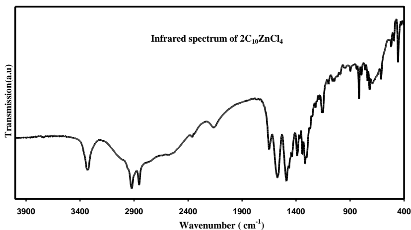
Fig-1. Infrared spectrum of 2C 10 ZnCl 4 .
