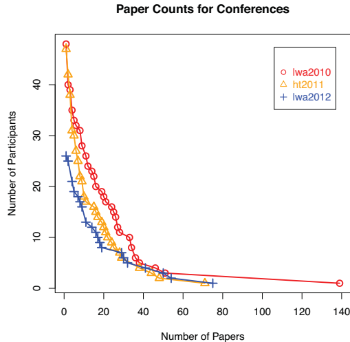
Figure 2: Distribution of the number of papers for each participant analyzed at the three conferences. The x -axis displays the minimum number of papers, the y -axis the number of participants having at least this paper count.
