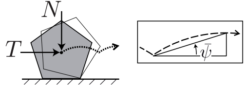
FIGURE 2. Trajectory of the center of mass of the polygon (dashed line) and definition of the mean dilatancy angle \bar{\psi} .
