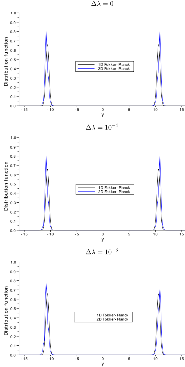
Figure 6. Distribution function comparison along y . The computed marginals of the 2D problem (blue line) at time t = 200 ms and the corresponding solution of the 1D reduced problem (black line) at the same time show a good agreement. In this test we have chosen the bifurcation parameter w_+ = 2.45 , the standard deviation \beta = 0.3 and the bias \Delta\lambda takes the values 0, 10^{-4} and 10^{-3} .
