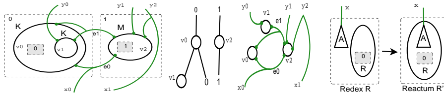
Fig. 1: A Bigraph G
