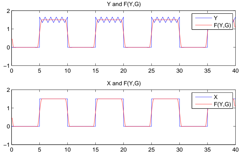
Figure 3: Filtering by using thresholding methode.
