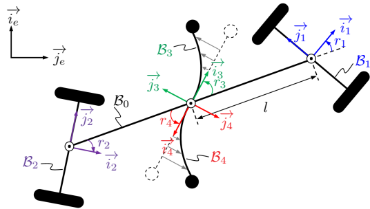
Fig. 4. Frames and parametrization of an elastic snake-board
