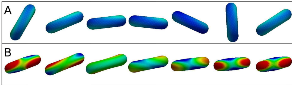
Figure 13: (color on-line) Dynamics of RBCs in simple shear flow. Color by Lagrange multiplier \zeta . Snapshot A: tumbling. Snapshot B: tank-treading (with some breathing and oscillations of orientation). Changes in the Lagrange multiplier \zeta due to membrane tank-treading are clearly seen.
