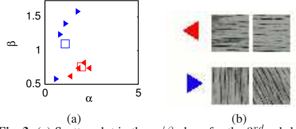
Fig. 3. (a) Scatter plot in the \alpha/\beta plane for the 3^{rd} sub-band and (b) example of samples from each cluster.
