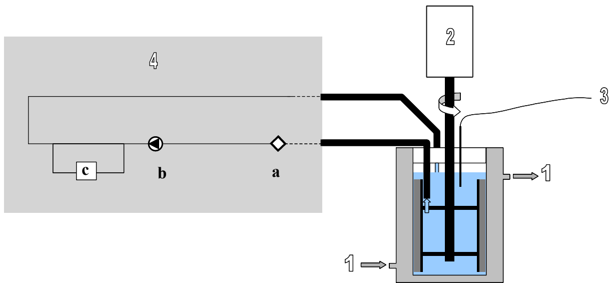
Figure 1: Schematic representation of the experimental set-up. (1): Primary refrigerant circulation; (2): Stirring and scraping system; (3): Temperature sensor; (4): Circulation loop (a: flowmeter; b: slurry pump; c: differential pressure transducer)
