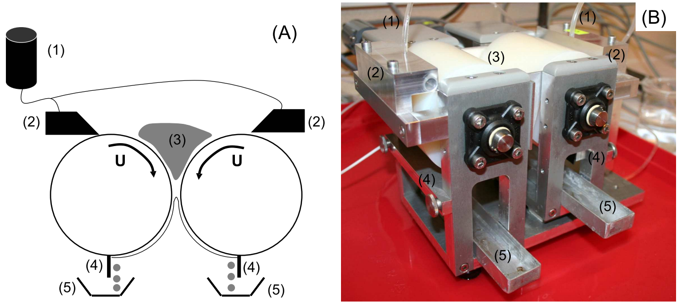
Figure 5: Pharyngeal peristalsis simulator: (1) saliva feed, (2) slot coater, (3) food bolus, (4) scraper, (5) collector.
