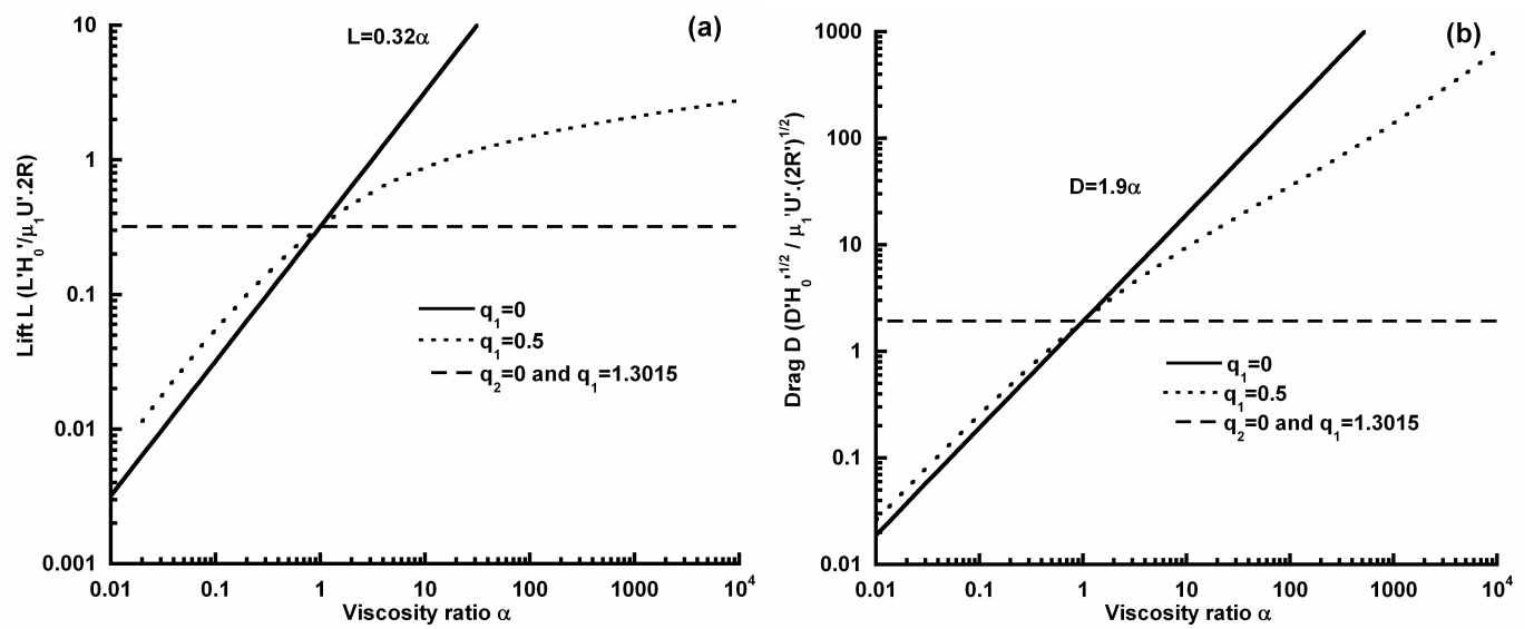
Figure 9: Dimensionless lift L (a) and drag D (b) as a function of the viscosity ratio \alpha for different saliva flow rates q_1 at imposed gap and velocity ( Ca_m = 1000 ).
