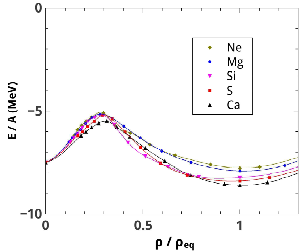
FIG. 1: (Color online) Equation of state for a choice of self-conjugate nuclei (EOS-A) as a function of average density scaled by the one at equilibrium, see text for detailed definition.
