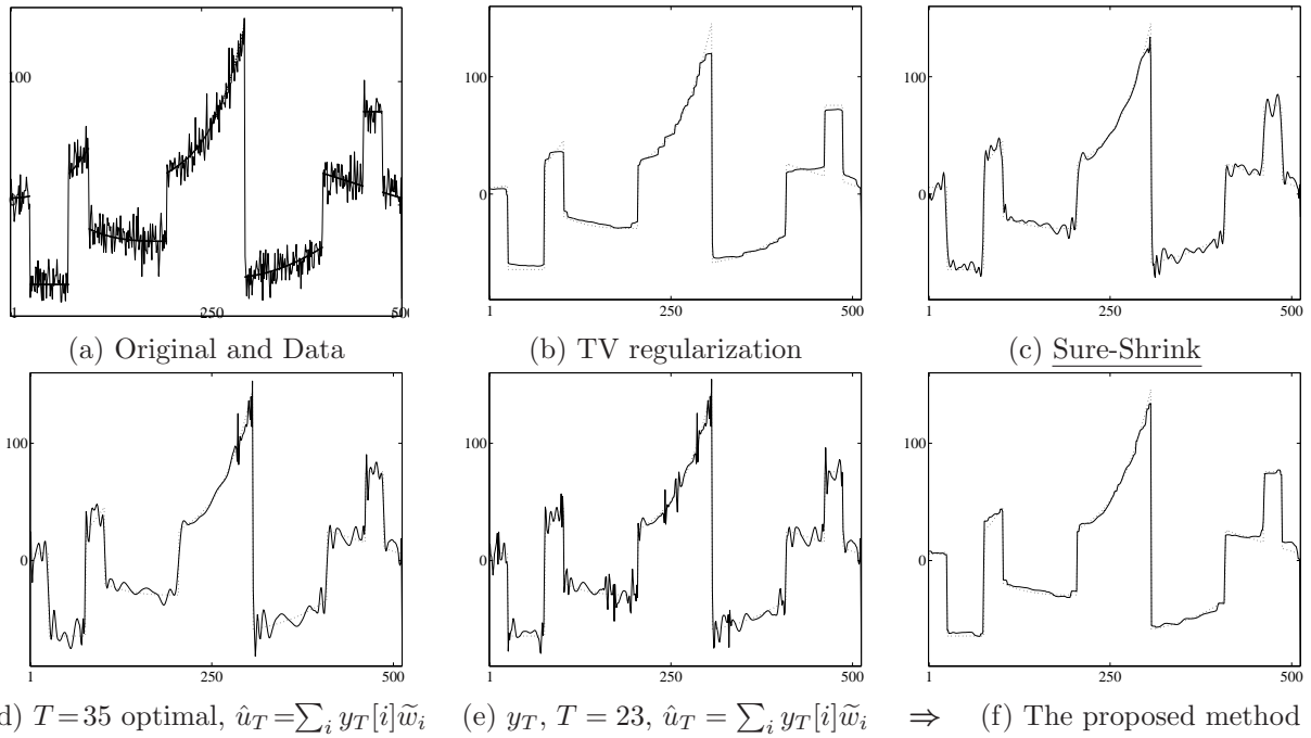
Figure 20: Methods to restore the noisy signal in (a). Restored signal (—), Original signal (- -).
