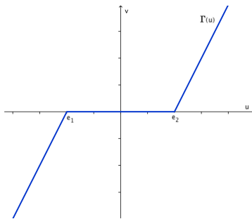
FIGURE 1. A typical graph \Gamma
