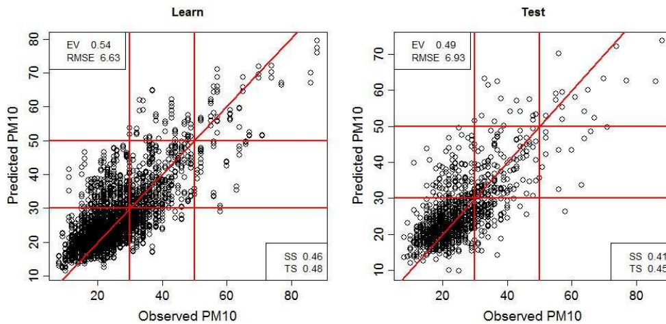
Fig. 6. Performance: predicted versus observed PM_{10} plots, from Learn (on the left) to Test (on the right) on REP Station.
