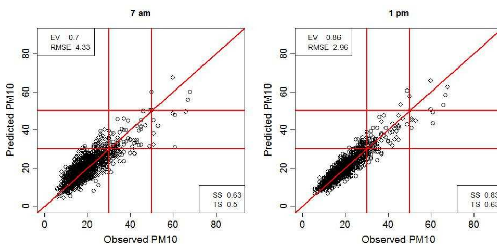
Fig. 9. Forecasting performance at 7 a.m. on the left and at 1 p.m. on the right for the urban station JUS.
