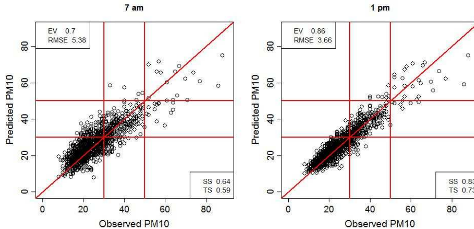
Fig. 10. Forecasting performance at 7 a.m. on the left and at 1 p.m. on the right for the urban station REP.
