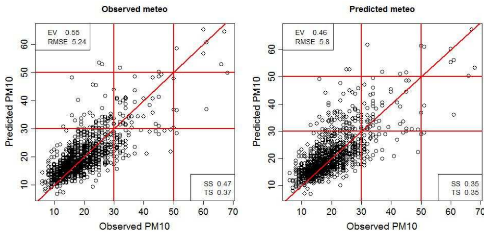
Fig. 7. Performance: predicted versus observed PM_{10} plots, from observed meteo (on the left) to predicted meteo (on the right) on JUS Station.
