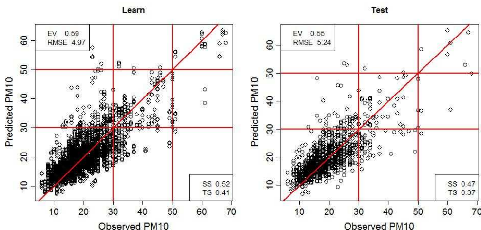
Fig. 5. Performance: predicted versus observed \text{PM}_{10} plots, from Learn (on the left) to Test (on the right) on JUS Station.
