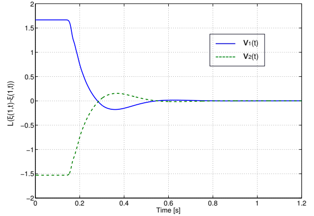
Fig. 9. The time evolution of the observer input v(t) .
