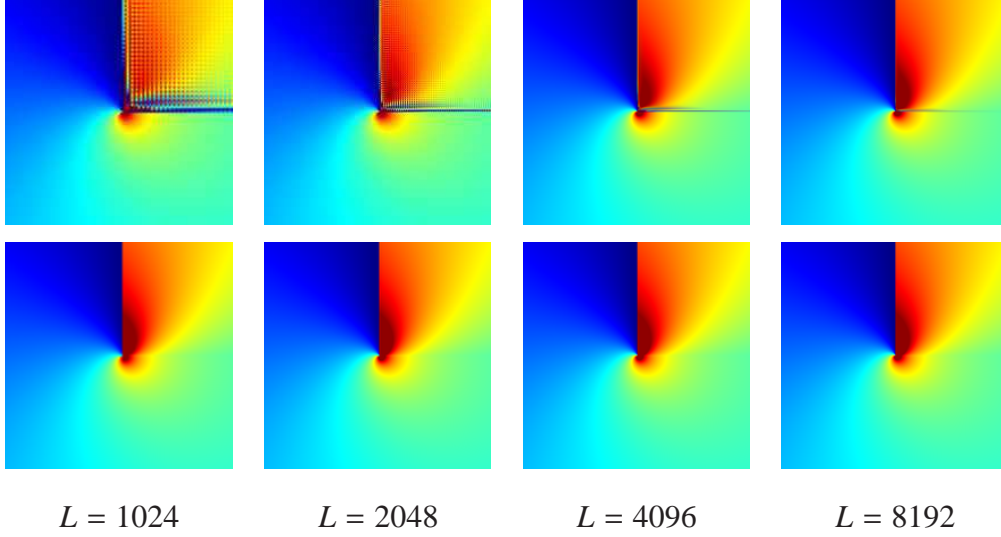
Figure 3. Four-cell microstructure of Figure 2. Maps of the vertical current component J_1(x, y) in the region -0.05L \leq x, y \leq 0.05L , for increasing resolution L (as indicated). Top: with continuous Green operator \mathbb{G}^0 . Bottom: with discrete operator \widetilde{\mathbb{G}}^0 .
