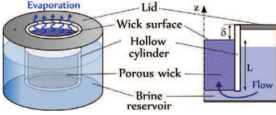
Fig. 1: (Colour on-line) Sketch of the experiment. A column of porous medium of height L = 35 mm is set in a hollow cylinder (38 mm in diameter and 50 mm in height). The bottom portion of the sample is submerged in a near saturated aqueous solution of sodium chloride ( C = C_0 = 25 g NaCl/100 g solution; the saturation concentration is C_{sat} = 26.4 g NaCl/100 g solution). The aqueous solution level in the brine reservoir is such that the medium remains saturated during the experiment duration owing to capillary rise. The system is set in a cylindrical enclosure (not shown) of controlled relative humidity ( RH \approx 7\% ) and temperature ( T \approx 22.4^\circ\text{C} ) (see [7] for more details). The distance \delta between the porous medium surface and the cylinder entrance rim is 15 mm.
