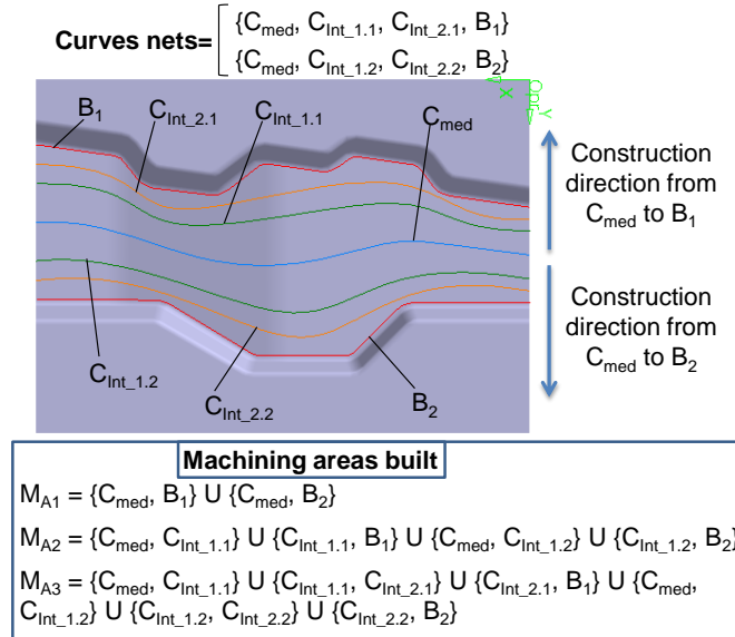
Fig. 10 Composed machining areas ( K=0.5 )
