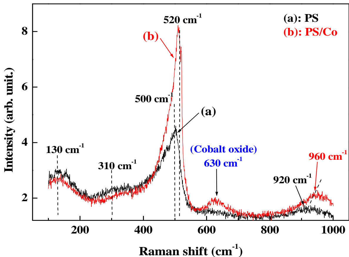
Figure 3: Raman spectra of unannealed PS and PS/Co.
