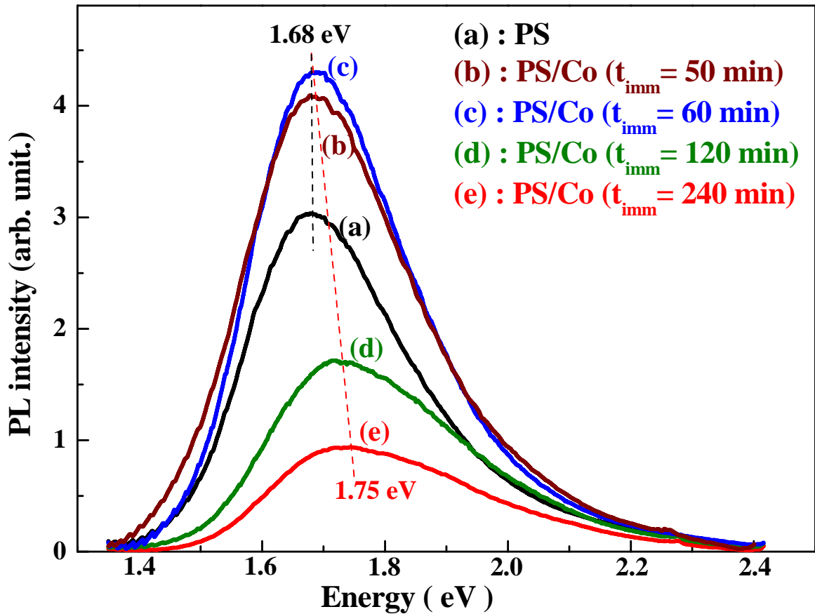
Figure 6: PL spectra of PS and PS/Co samples with different immersion durations in CoCl 2 aqueous solution.
