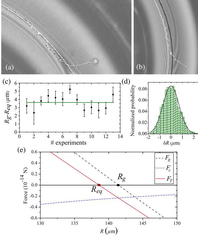
FIG. 3 (color online). Example of trajectories of beads on the air-oil interface with contact angle (a) \theta = 0^\circ and (b) \theta = 30^\circ . The black line is the locus of the radial minimum height of the interface ( R_g ). The white circle corresponds to the final equilibrium radius R_{eq} of the bead. Note also the visible thermally driven fluctuations \delta R around R_{eq} . (c) Deviation R_g - R_{eq} for various experiments made with different beads with \theta = 30^\circ \pm 2^\circ and cuvettes with \langle \delta R^2 \rangle error bars. (d) Typical probability distribution function vs \delta R and best fit with a normal distribution. (e) Curvature force F_c , gravity force F_g , and the resulting total force F_T vs R . F_c and F_g are plotted using \gamma = 28 \text{ mN m}^{-1} [25], \phi_0 = 53^\circ , \theta = 30^\circ , R_1 = 100 \mu\text{m} , R_2 = 200 \mu\text{m} , a = 2 \mu\text{m} , and m_f = 5.75 \times 10^{-11} \text{ g} .
